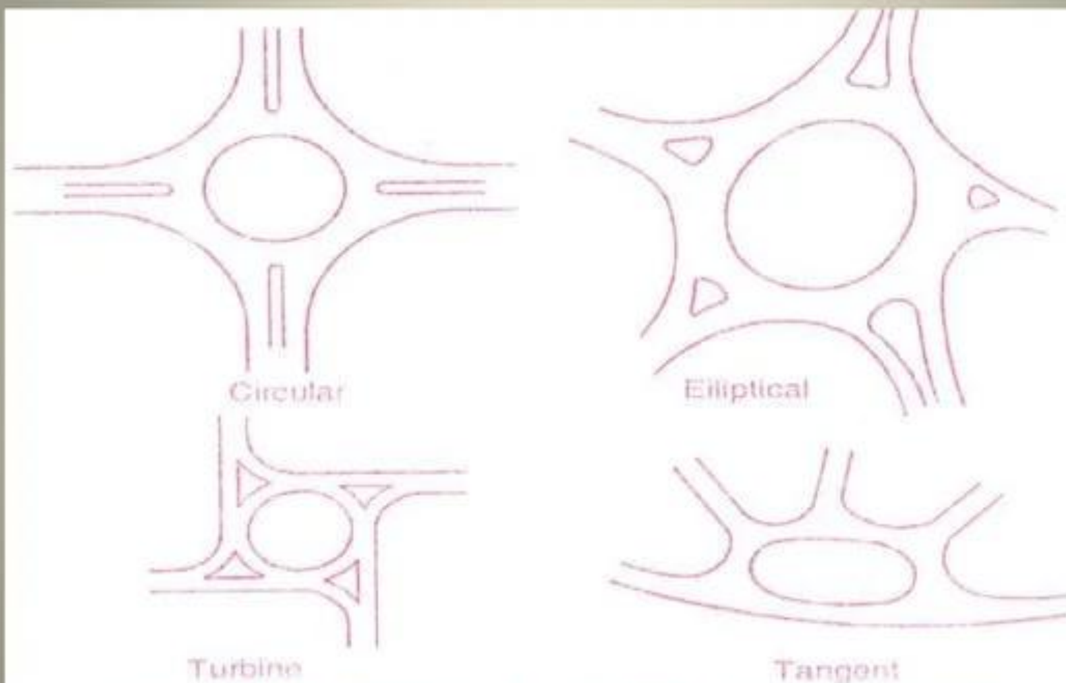
Fig. 12.30 Types of rotary intersections
