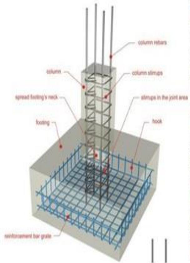
|| || Isolated RCC Footing
