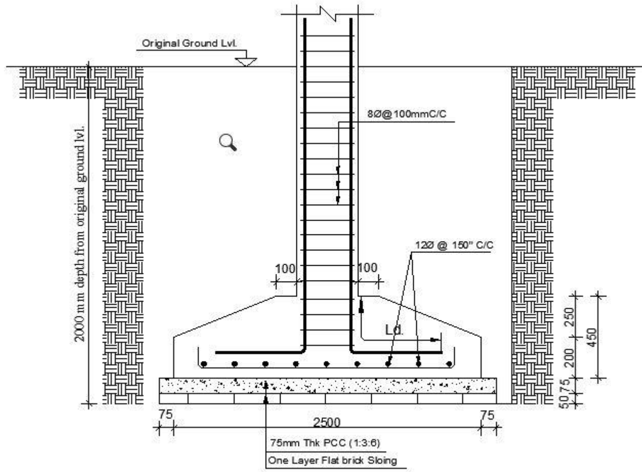
FOOTING "F1" SECTION AT (A-A)
