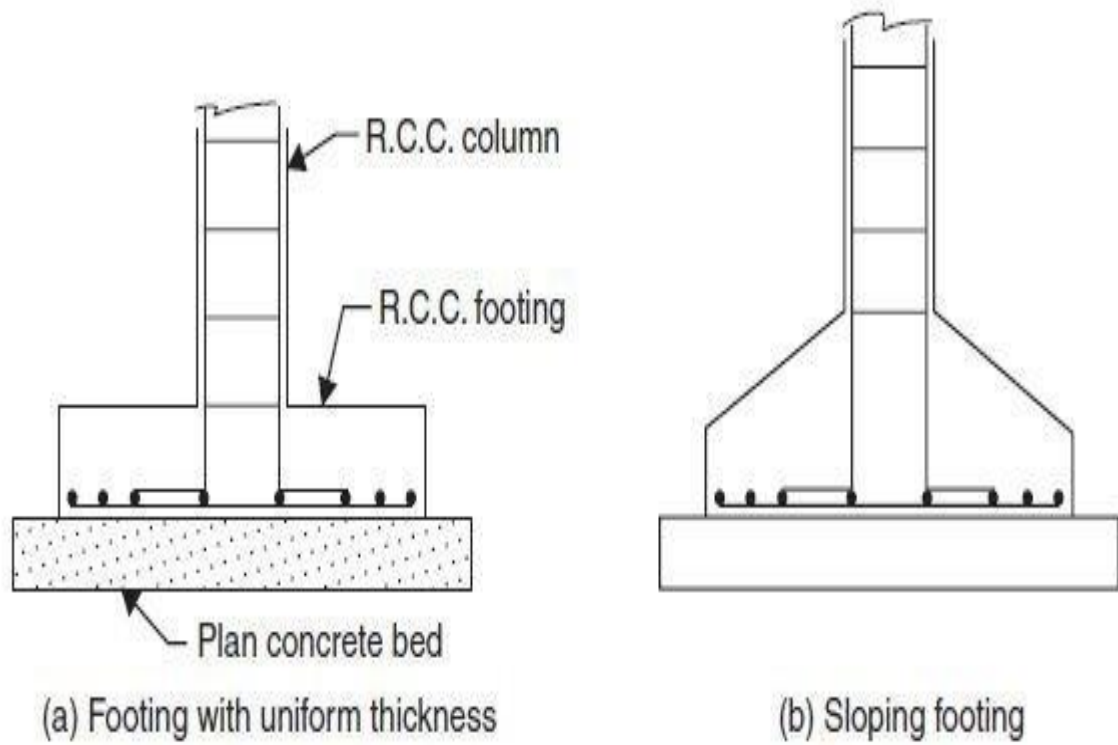
Fig. 7.3. Isolated R.C.C. footing
