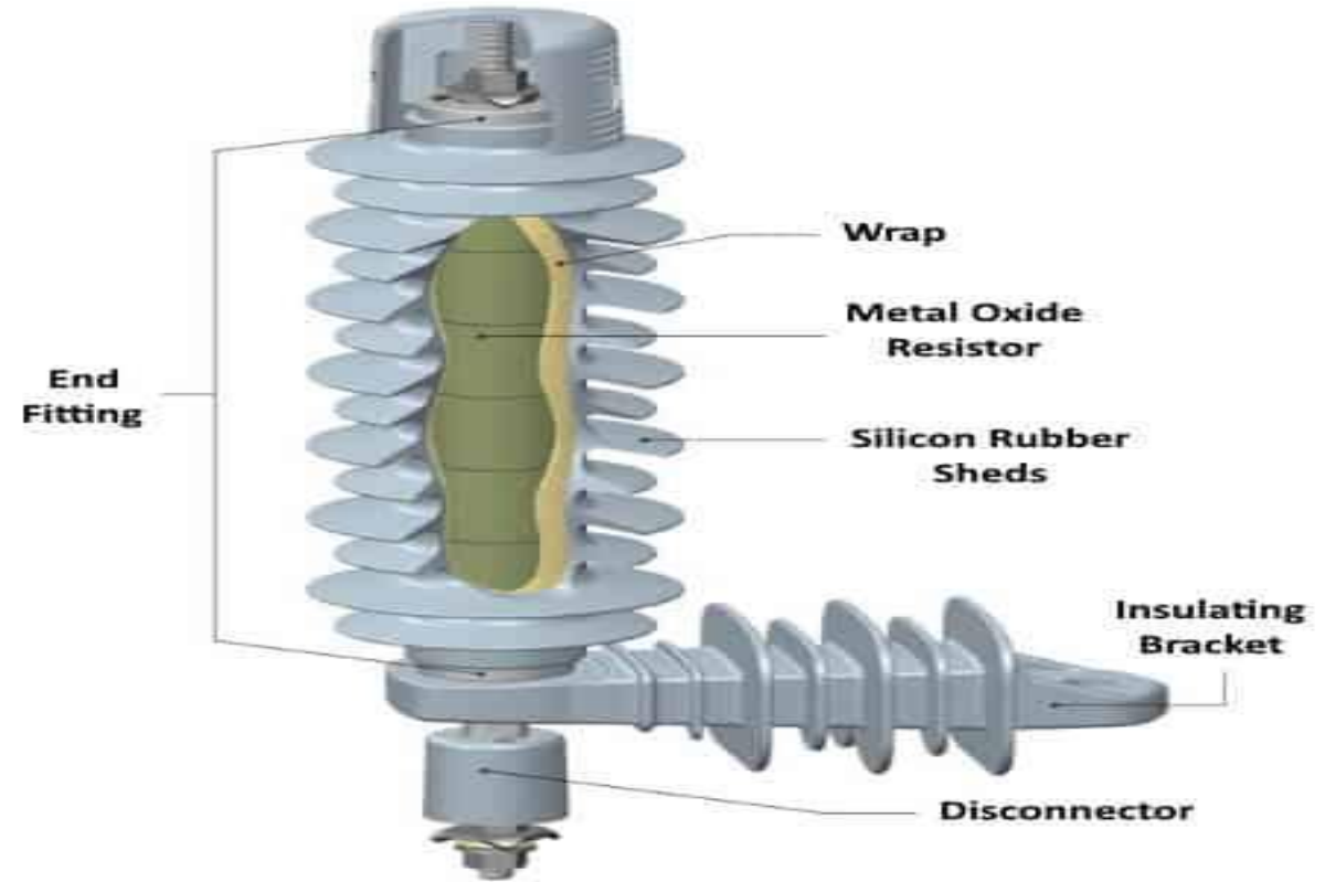
Surge Arrester
