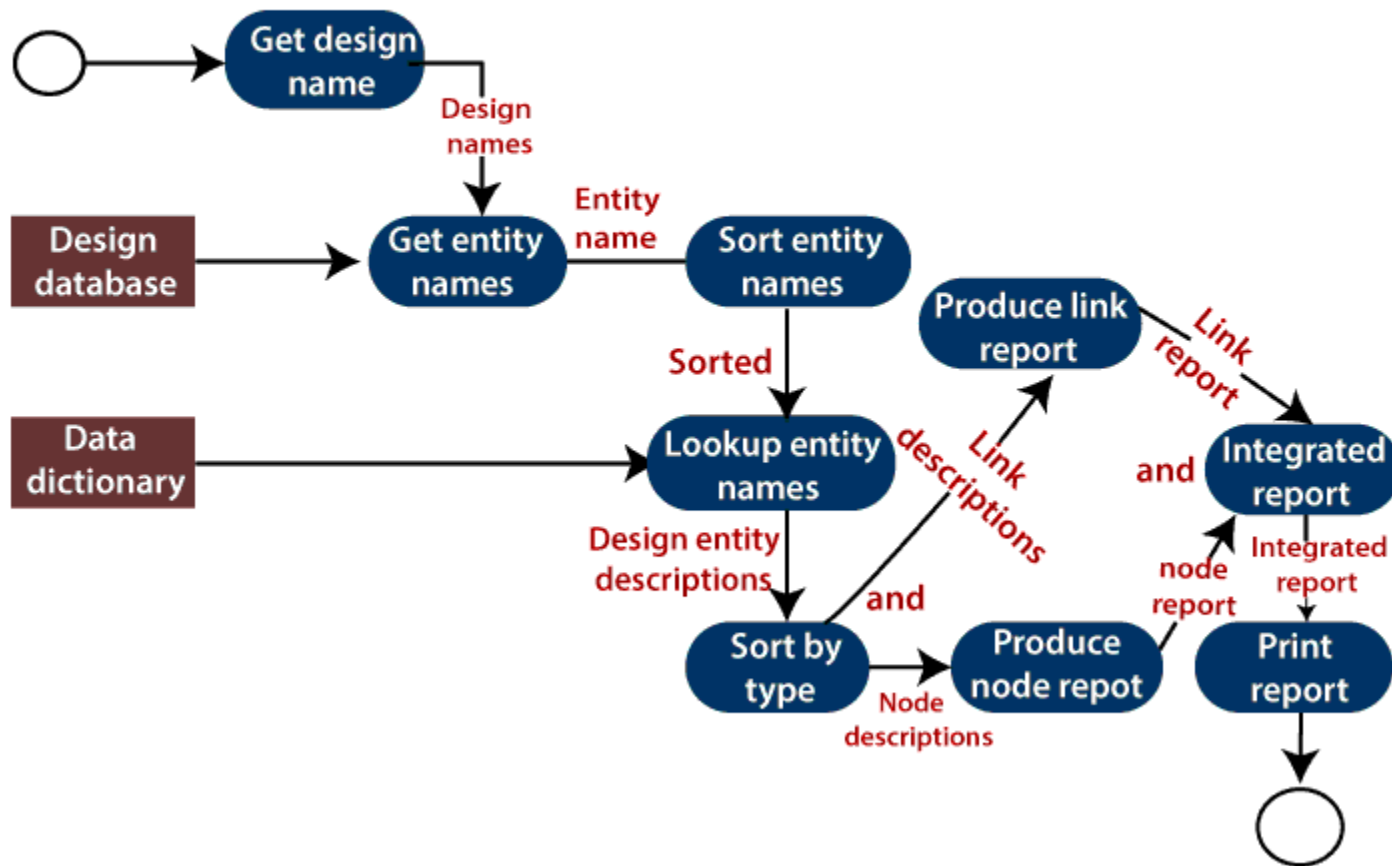
Data flow diagram of a design report generator
