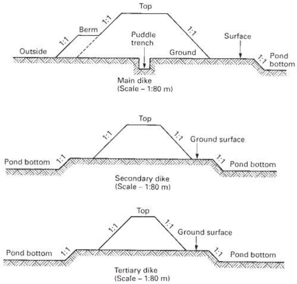
Fig. 6.4 Cross-sections of some typical types of dikes.
